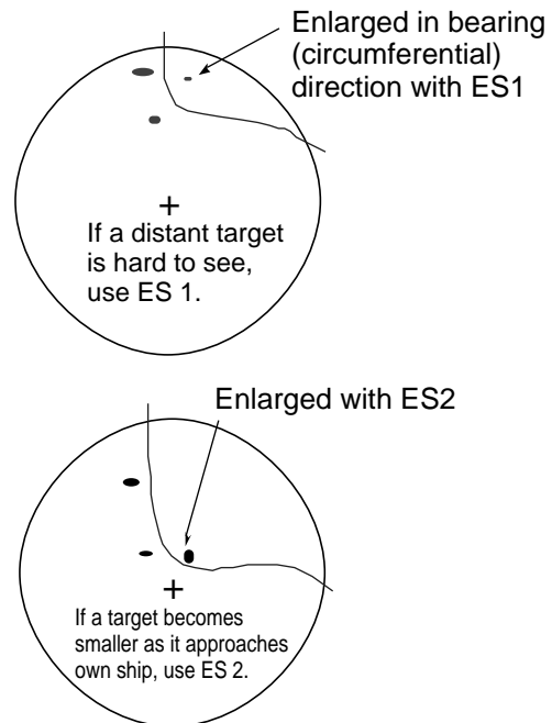
Figure 1-10 Echo stretch
